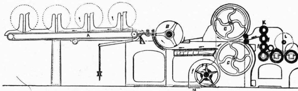
SECTIONAL VIEW
