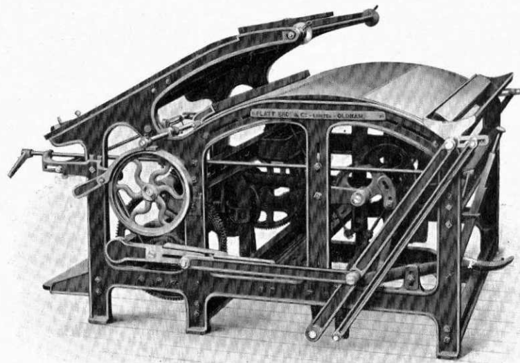
CLOTH-FOLDING MACHINE
