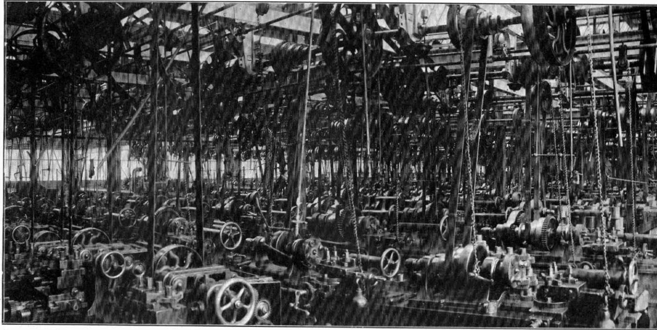
A PORTION OF THE GENERAL TURNING DEPARTMENT
